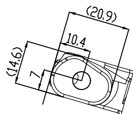
A SECTION
