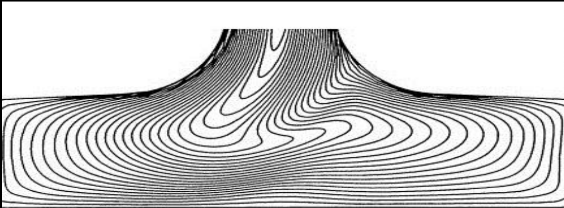
金屬流向分析剖面圖(ATV 羊角臂和輪椅零件) Analysis of metal flow of a cut surface (e.g. ATV knuckle and wheel chair parts).
